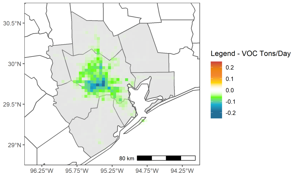
Figure 1-24: Difference in On-Road VOC Emissions for the June 12 Episode Day Between 2026 and 2019 in HGB
